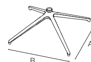
07 Maui Lounge - Lounge Plus | Base Kylie in alluminio a 4 razze - Ø840 Maui Lounge - Lounge Plus | Kylie 4-spokes aluminium base - Ø840
